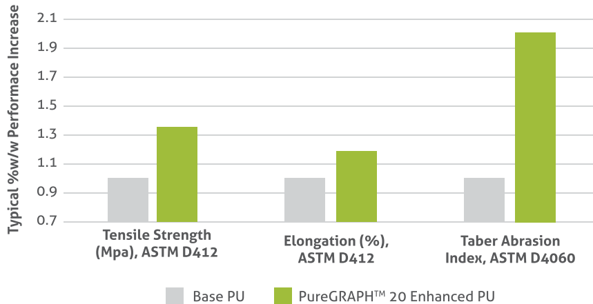
Fig. 3. Performance Results of PureGRAPH™ enhanced Polyurethanes.
