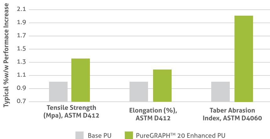
Fig. 3. Performance Results of PureGRAPH™ enhanced Polyurethanes.
